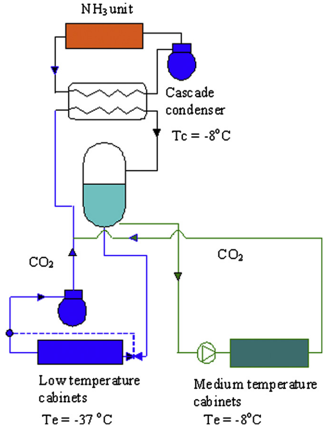
Fig. 9. Schematic diagram of NH 3 /CO 2 cascade system with CO 2 at the medium temperature and low temperature levels.
