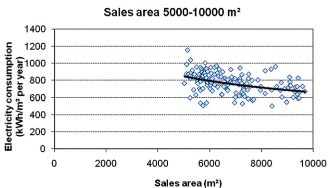
Fig. 4. Electrical energy intensity of supermarkets of sales area between 5000 m 2 and 10000 m 2
