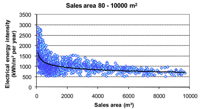
Fig. 5. Variation of electrical energy intensity of 2570 UK retail food stores with sales area from 80 m 2 to 10,000 m 2
