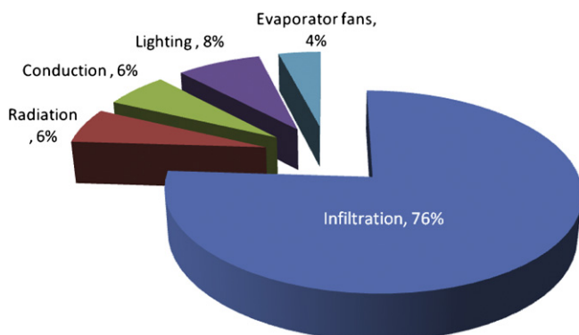
Fig. 14. Contributions to the load of a vertical multi-deck open front chilled food display cabinet.
