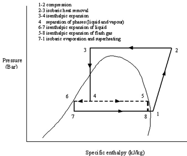
Fig. 11. P-h Diagram of medium temperature transcritical CO 2 system.
