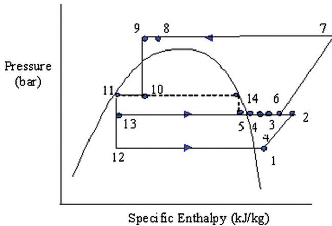
Fig. 13. P-h diagram of booster system.
