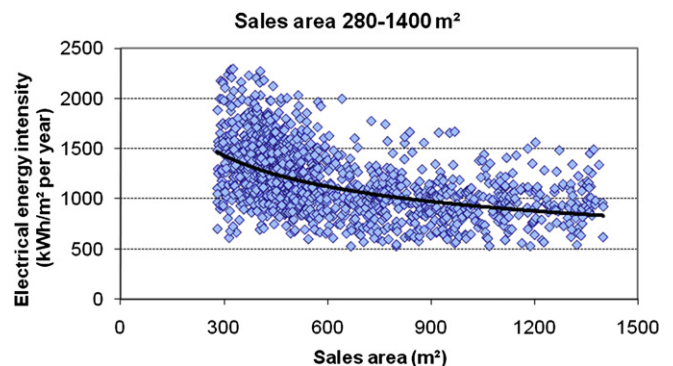
Fig. 2. Electrical energy intensity of supermarkets of sales area between 280 m 2 and 1400 m 2
