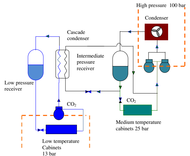
Fig. 10. Schematic diagram of all CO 2 cascade system.
