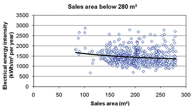
Fig. 1. Electrical energy intensity of convenience stores of sales area between 80 m 2 and 280 m 2
