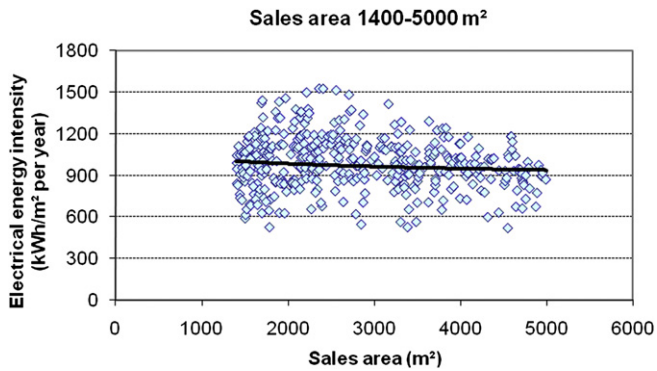
Fig. 3. Electrical energy intensity of supermarkets of sales area between 1400 m 2 and 5000 m 2
