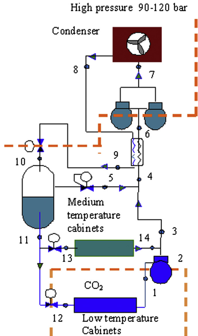
Fig. 12. Booster system with gas by-pass.
